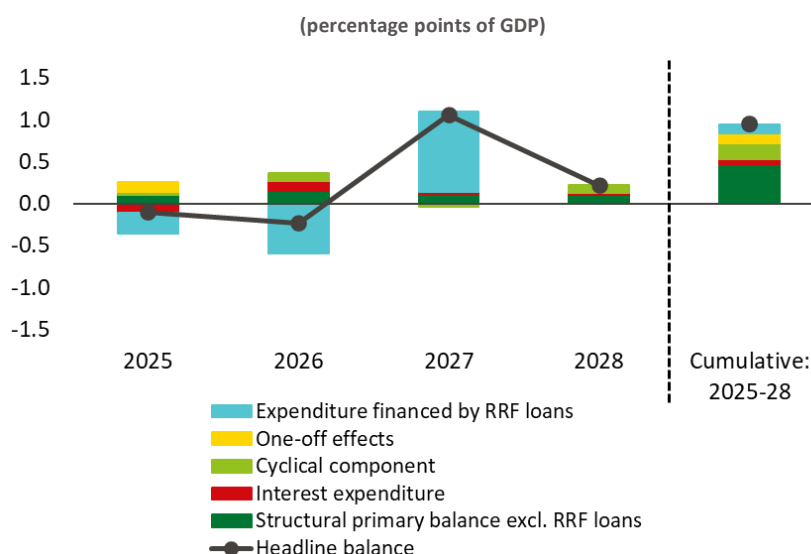
Figure 2.1. Breakdown of the change in the headline budget balance in 2025-2028
