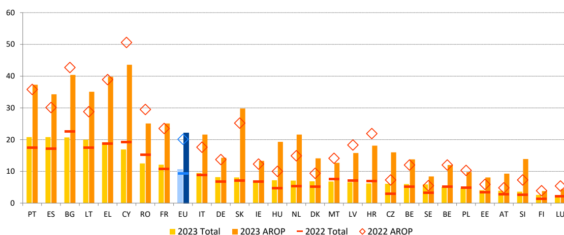
Figure 2.4.7: Energy poverty has been rising in the EU with significant variation across Member States
